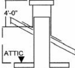
___ PITCHED ROOF FLASHING ATTIC
