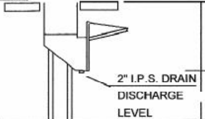
___ HOPPER W/ LEGS AND DRAIN
